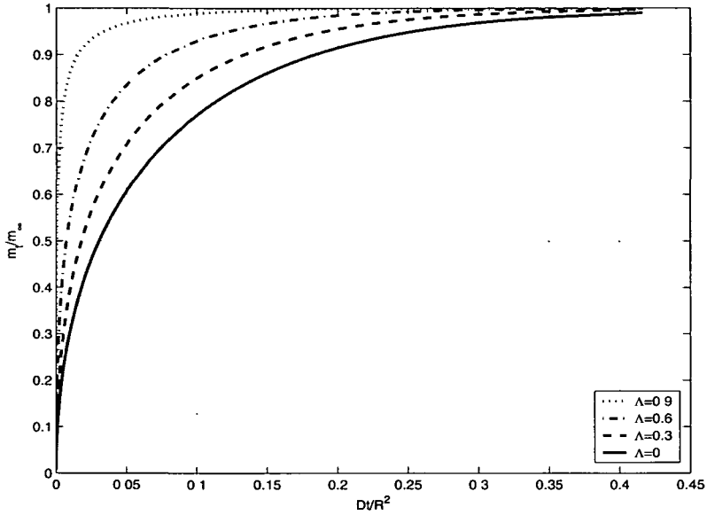
FIGURE 5. Theoretical uptake curves calculated by Equation (2.10) .
