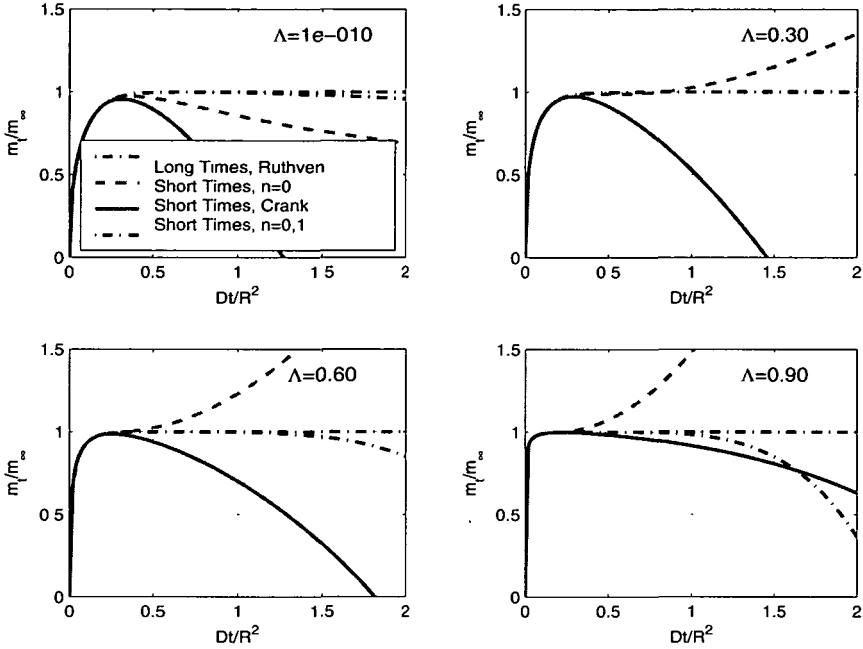
FIGURE 2. Long-time and short-time solutions for various \Lambda .
