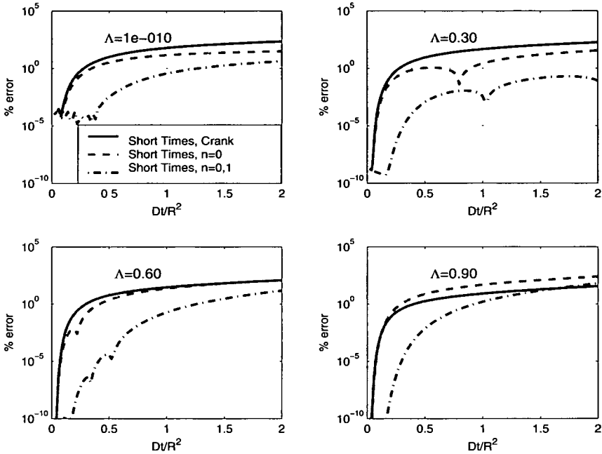
FIGURE 3. Relative error using short-time solutions for various \Lambda .
