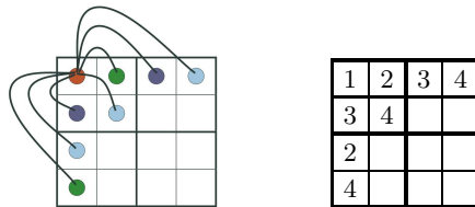
Figure 3: Part of the graph associated to Shidoku.
