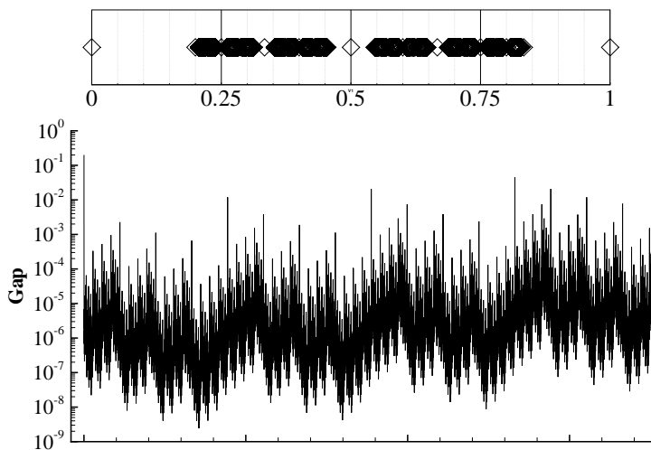
Figure 1: Distribution of elements of F(4) with b_0 = 0 with up to eight partial quotients, and the gaps between these elements.
