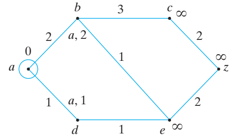
Figure 8.4.8 The first iteration of Dijkstra's shortest-path algorithm.
