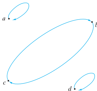
Figure 3.3.2 The digraph of the relation of Example 3.3.5.
