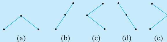
Figure 9.8.12 The five nonisomorphic binary trees with three vertices.
