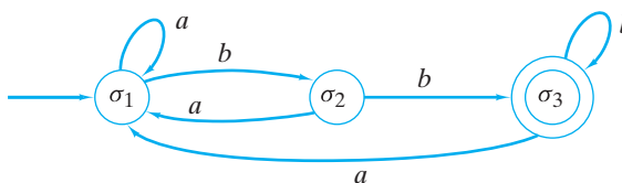
Figure 12.5.4 The finite-state automaton for Example 12.5.7 that accepts L .
