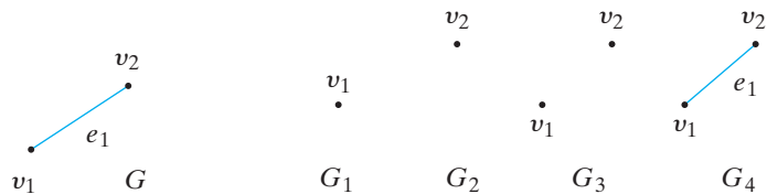
Figure 8.2.5 The graph for Example 8.2.10.
