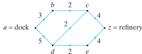
Figure 10.1.1 A transport network.
