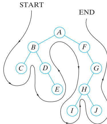
Figure 9.6.5 Preorder traversal.
