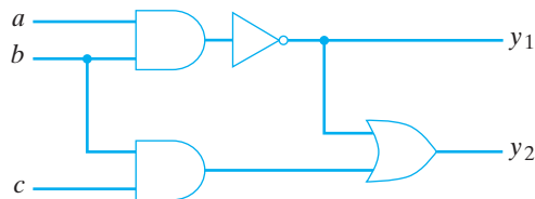
Figure 11.5.7 A combinatorial circuit with two outputs.
