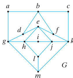
Figure 8.3.7 A graph with no Hamiltonian cycle.
