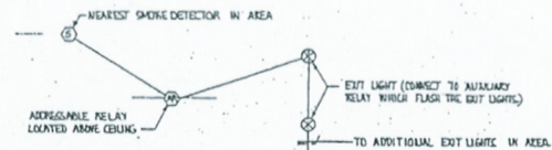
TYPICAL EXIT LIGHT FLASHER CIRCUIT DIAGRAM NOT TO SCALE
