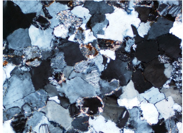
Thin section of Gowlaun matrix
