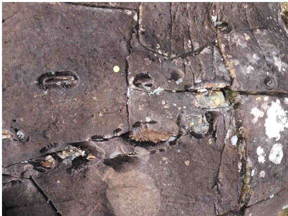
Lettergesh Fm. outcrop features; elongated holes indicate bedding surface
