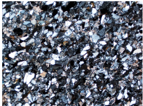
Thin section of a Kilbride Fm. sample
