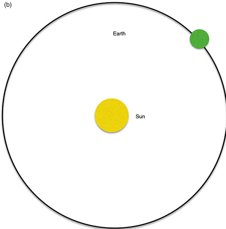
Figure 1. (a) Typical textbook illustration of a planet's orbit and (b) Earth's actual orbital.
